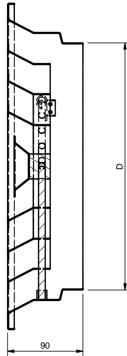
M-M (1:3)
